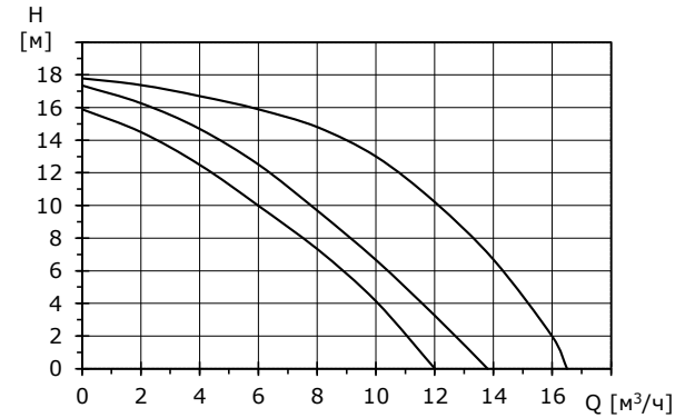
BASIC 40-16SF
