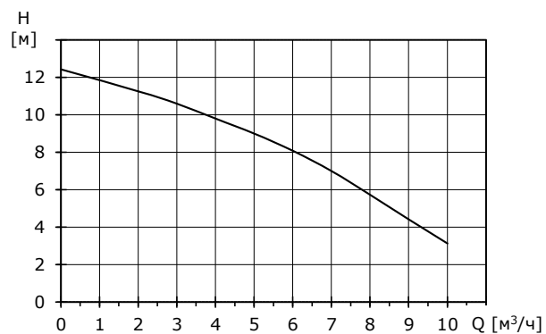
BASIC 32-12 180
